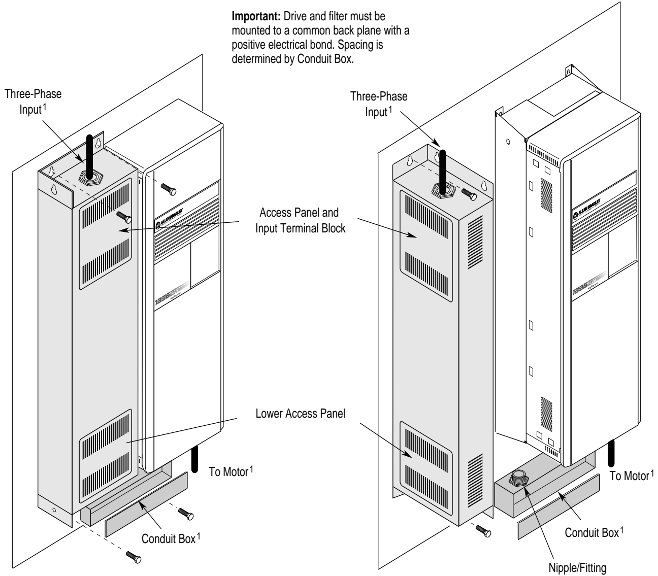
Figure 3 1336 PLUS, PLUS II, FORCE & IMPACT (Through-the-Wall Mounting) Frames D & E 2
