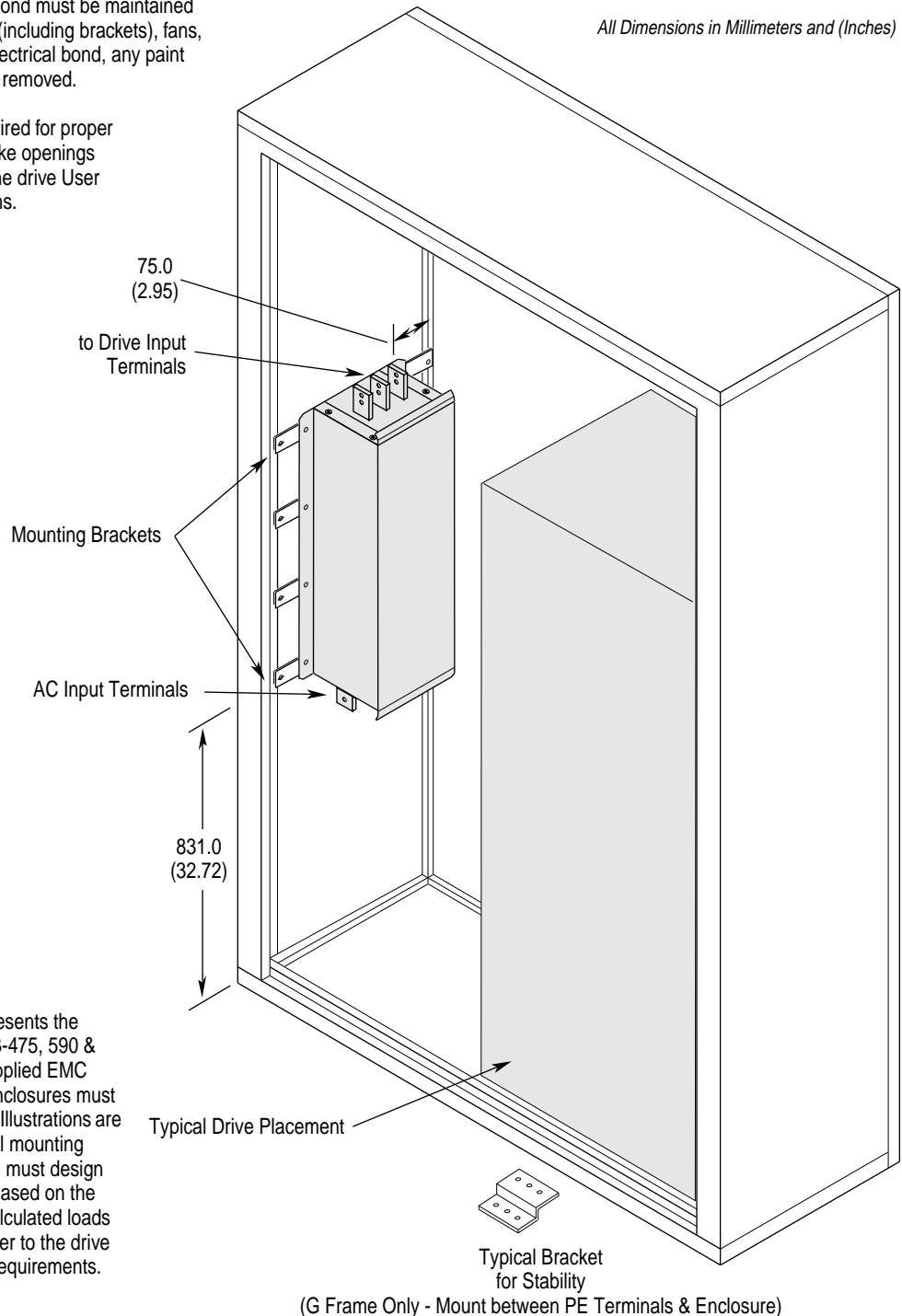
Figure 5 1336 PLUS, PLUS II, FORCE & IMPACT (Typical Filter Mounting)
