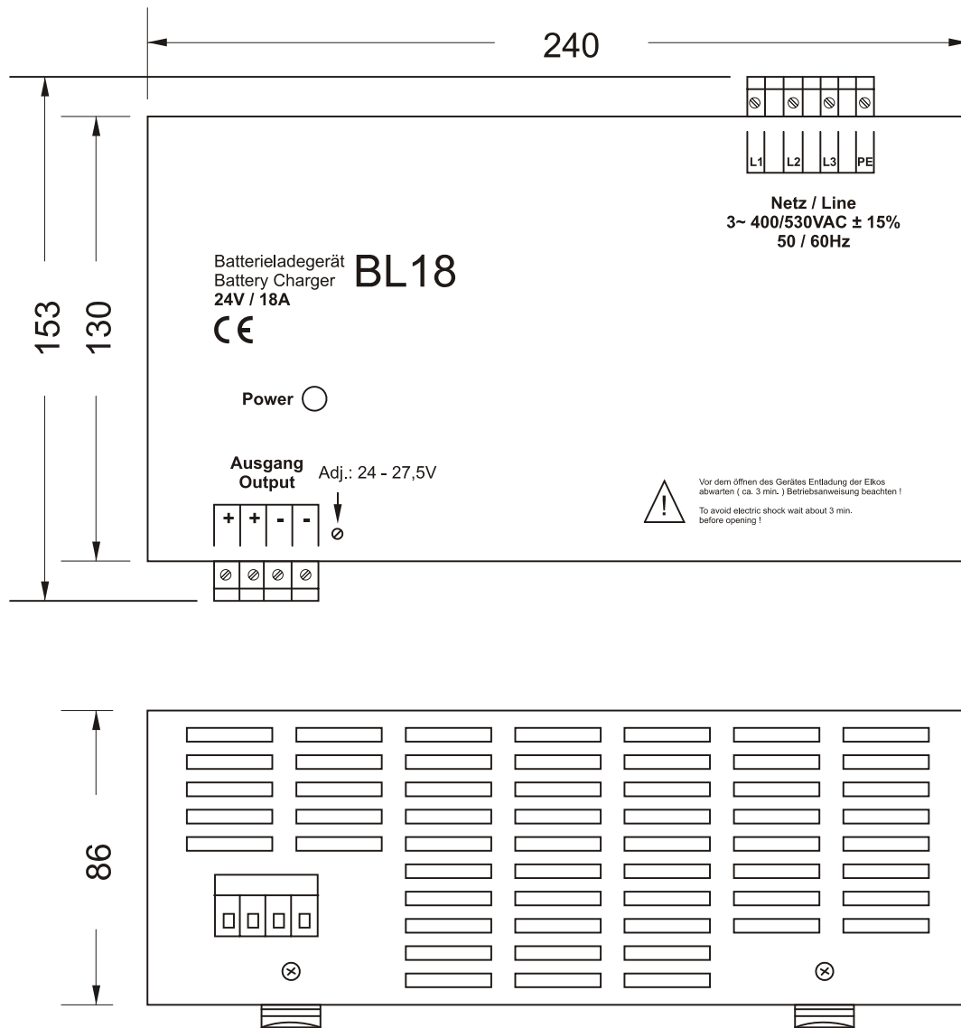
Figure 4.1: Housing dimensions
