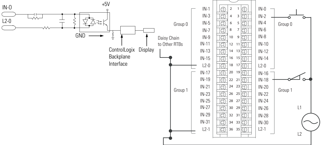
Simplified Schematic
