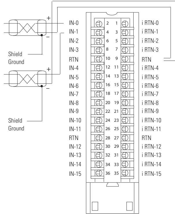
1756-IF16 Single-ended Voltage
