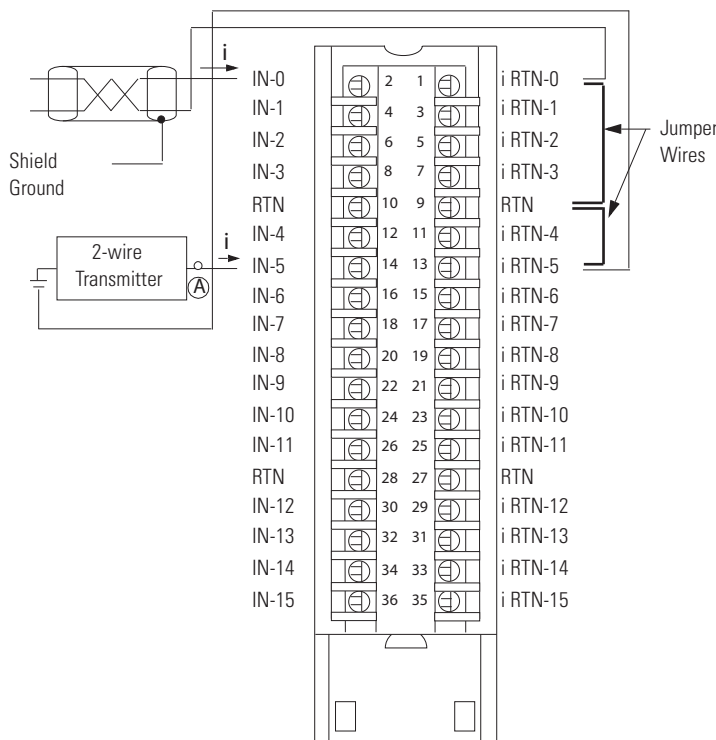
1756-IF16 Single-ended Current
