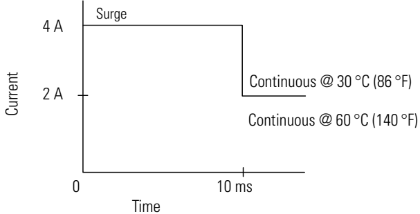
Surge Current Chart
