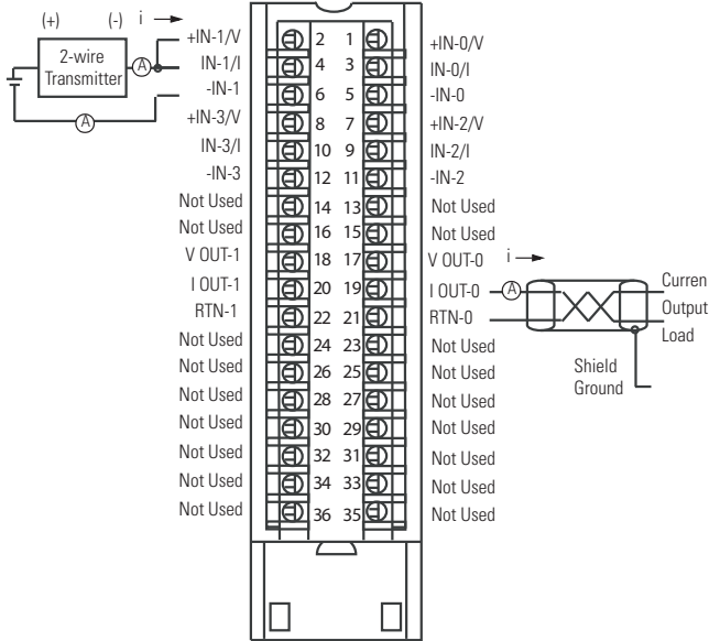
1756-IF4FXOF2F Current
