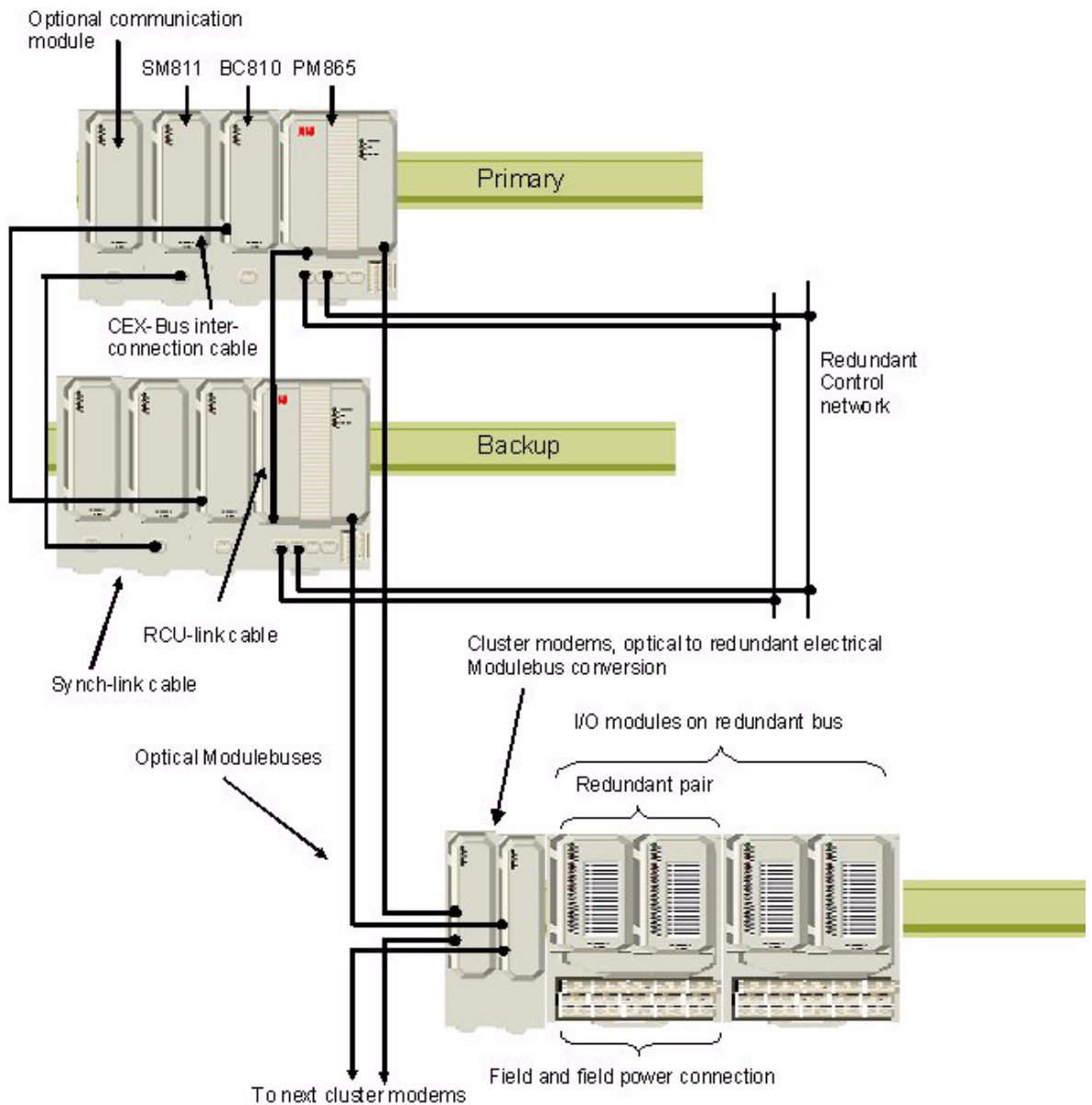
Figure 5. Redundant AC 800M HI System
