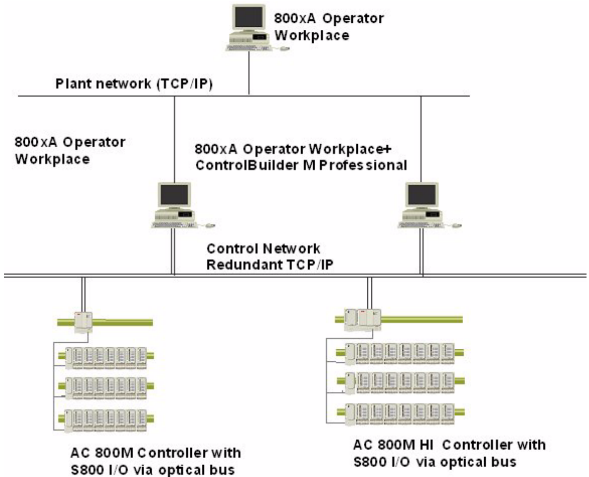
Figure 3. System Topology
